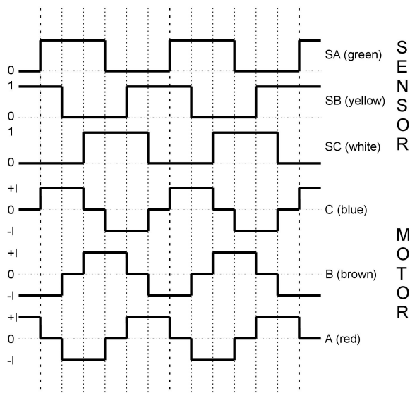
Typical commutation scheme of a BL-Motor, cw-direction
